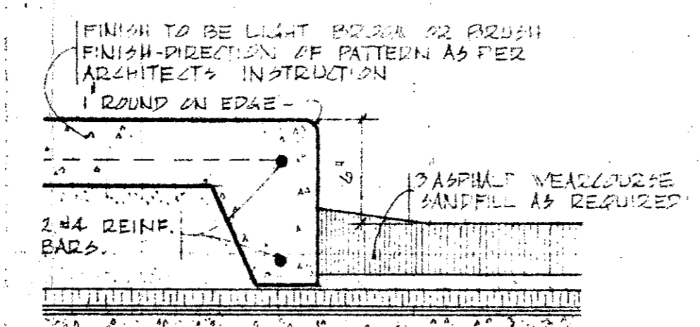
B. CONZ. WALK @ DRIVEWAY
