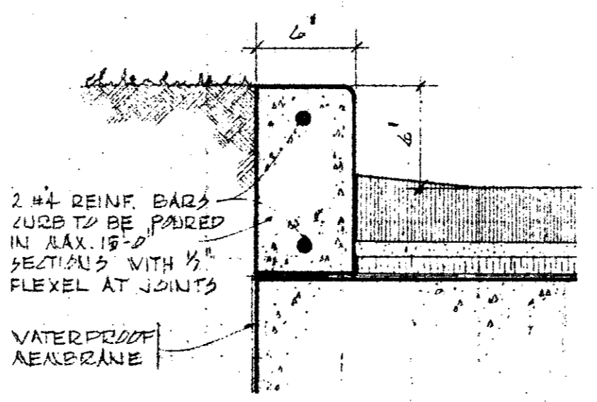
C. CONZ. CURB (ON STRUCTURE)
